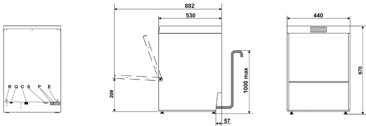
Glasswasher, 400x400 mm basket - UG401 Series
