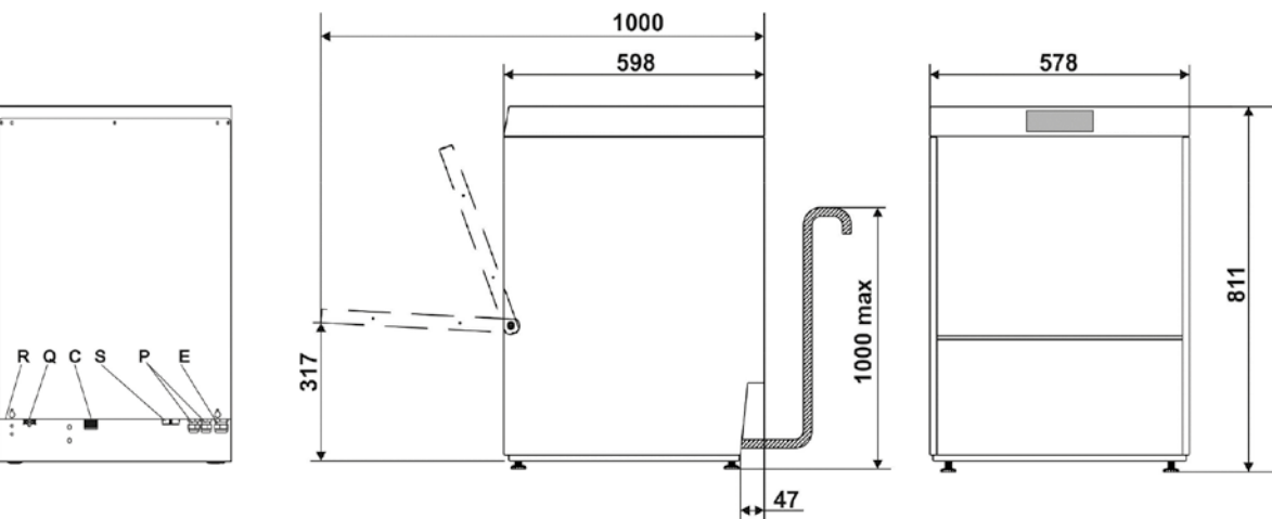
Dishwasher, 500x500 mm basket - UD503 and UD505 Series
