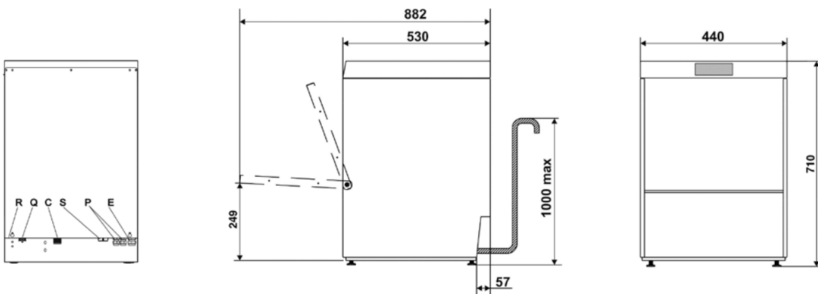
Glasswasher, 400x400 mm basket - UG403 and UG405 Series
