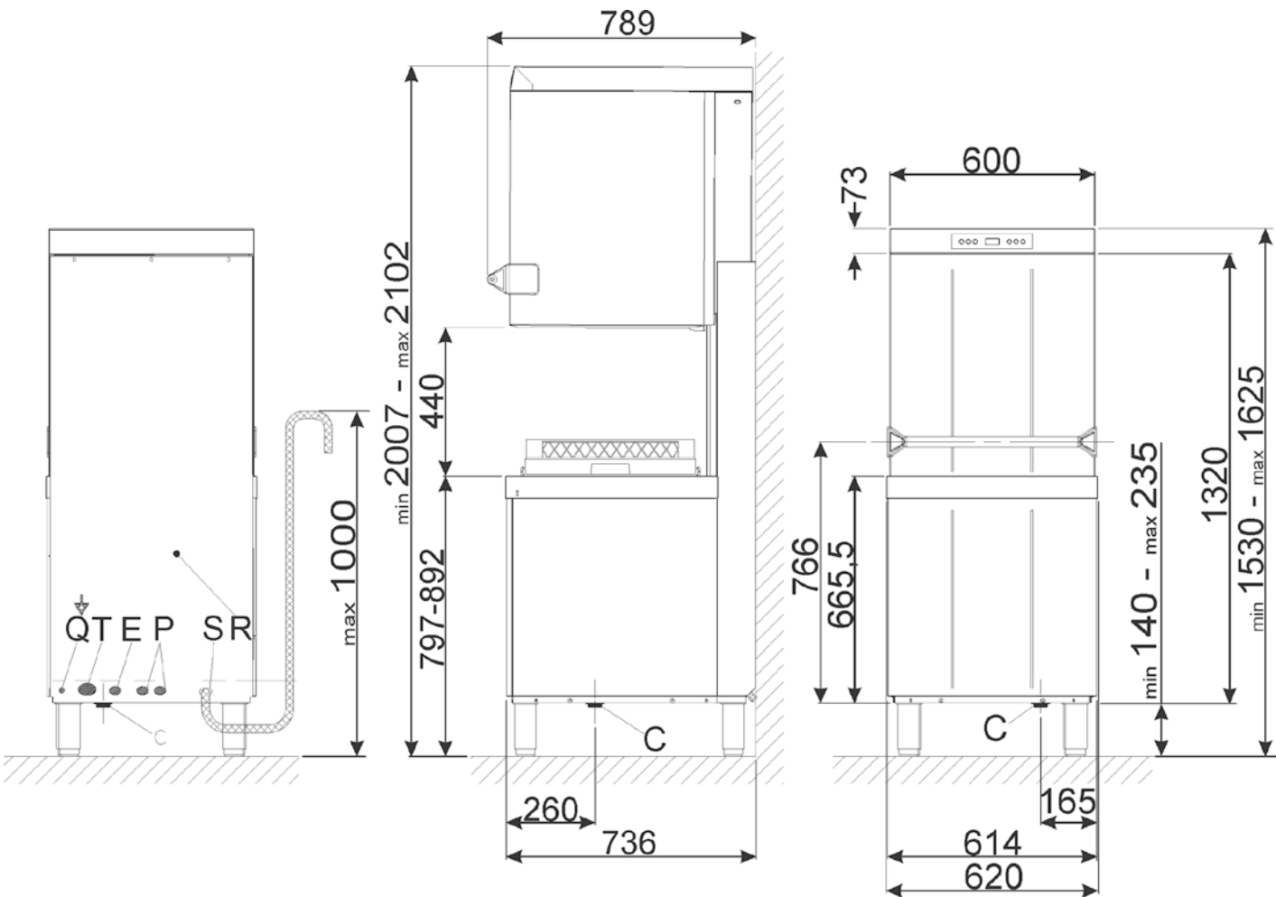
Hood, 500x500 mm basket - HTY503 and HTY505 Series
